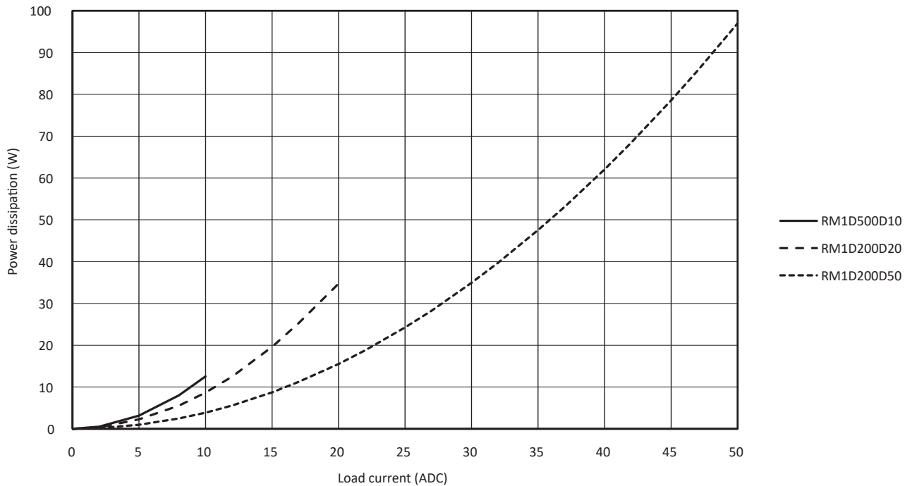
Fig. 9 Output power dissipation graph
